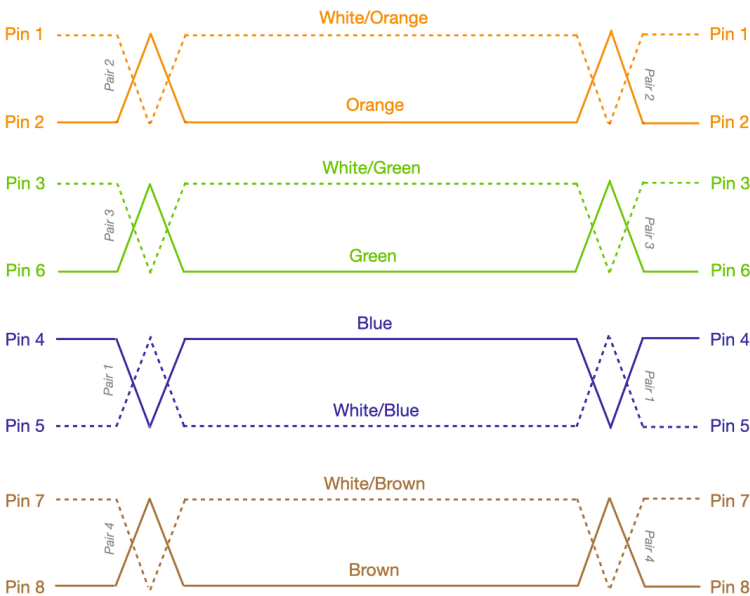
RJ45 - Side A Pin Out (T568B Wiring) RJ45 - Side B
